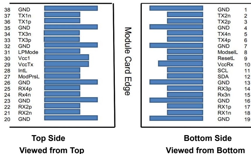
Figure 1 – QSF+ MSA-compliant 38-pin connector
